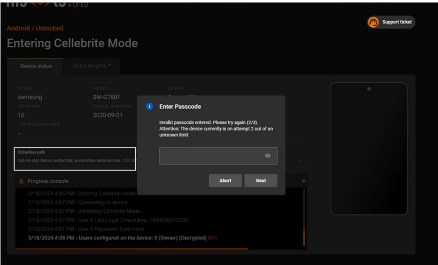
Figure 15: Cellebrite AFU mode interface showing “falcon_unlock”
